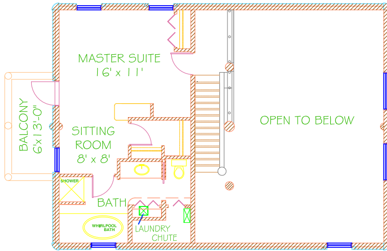
SECOND FLOOR PLAN COLORADO 1630 TOTAL sq.ft.
